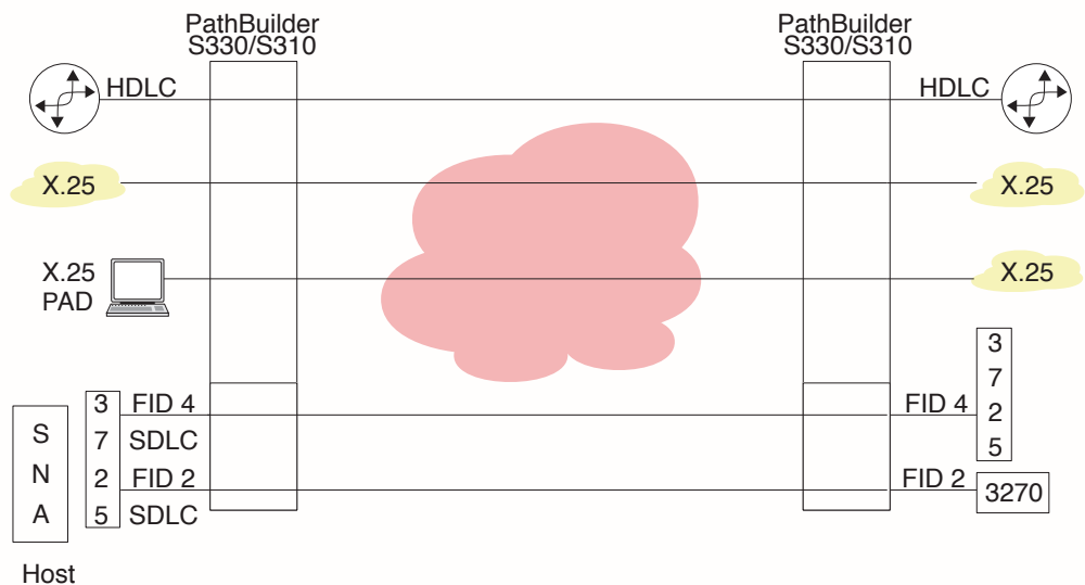
Figure 160 HDLC/SDLC Applications
