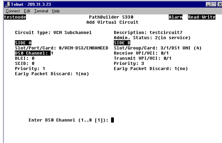
Figure 120 Configuring a VCM Subchannel Circuit
