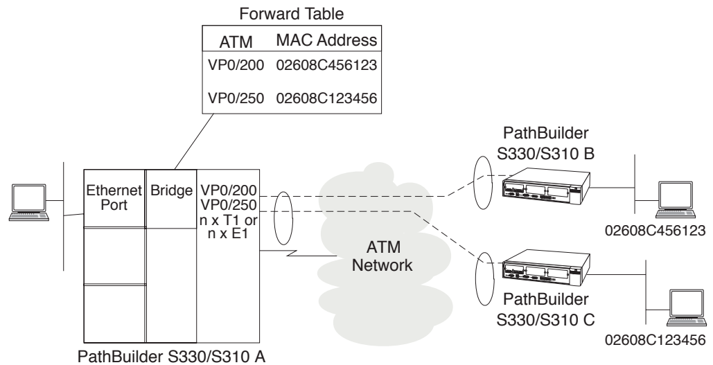
Figure 168 ATM Bridging
