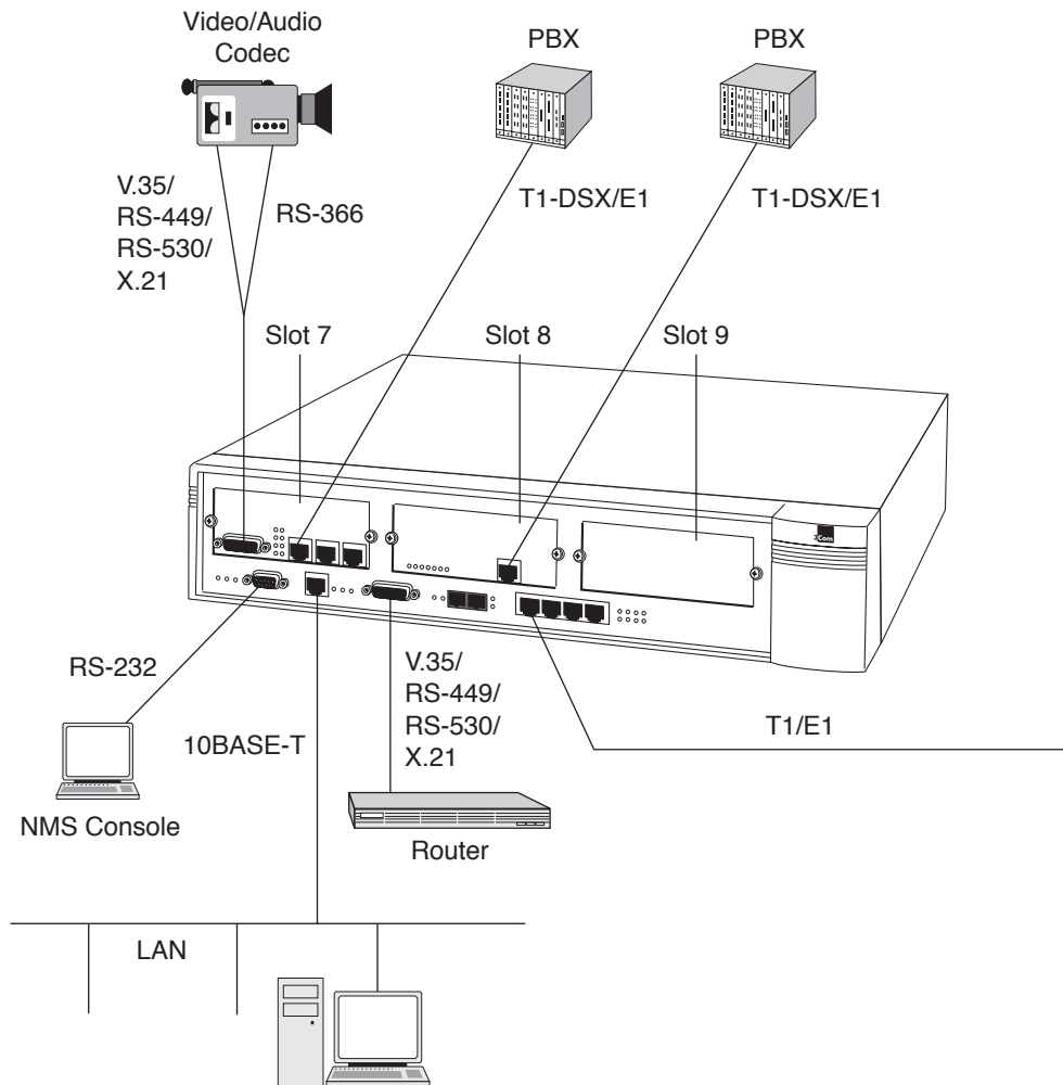
Figure 5 PathBuilder S310 Full System Configuration
