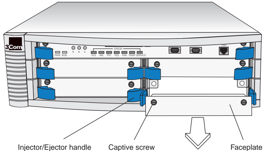
Figure 1 Removing the Blank Faceplate
