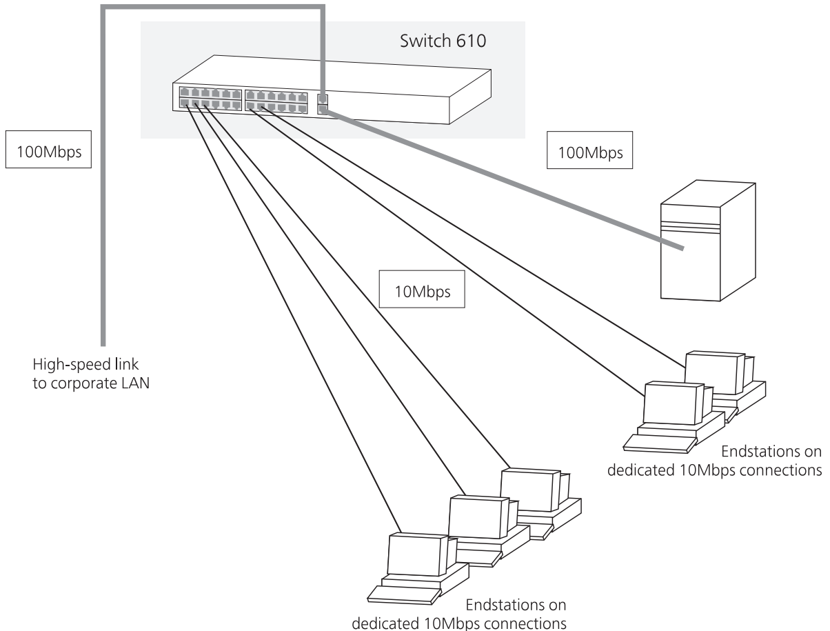
Figure 5 Using the Switch 610 in a desktop environment
