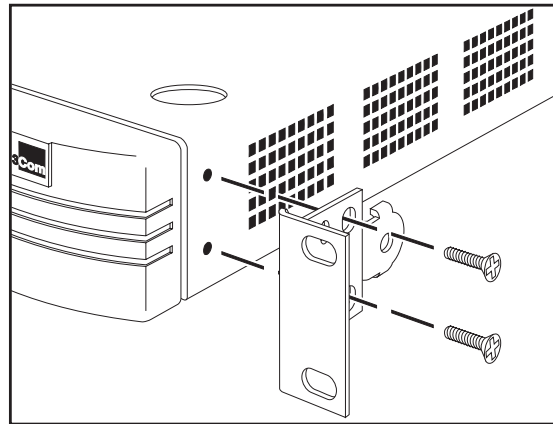
Figure 7 Fitting a bracket for rack mounting
