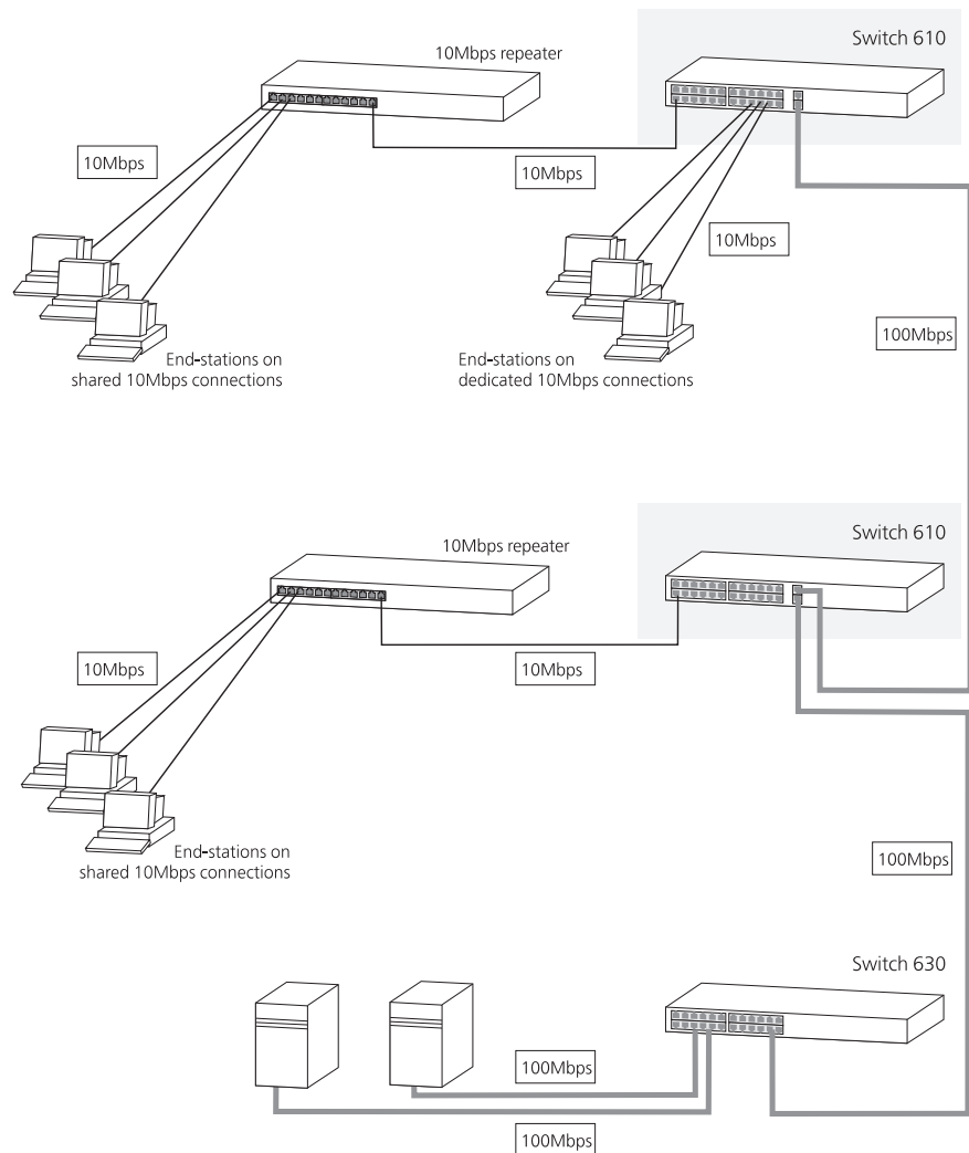
Figure 3 Using the Switch 610 to segment your network
