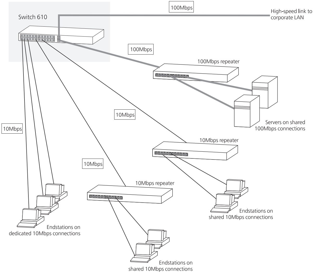
Figure 4 Using the Switch 610 to segment your network
