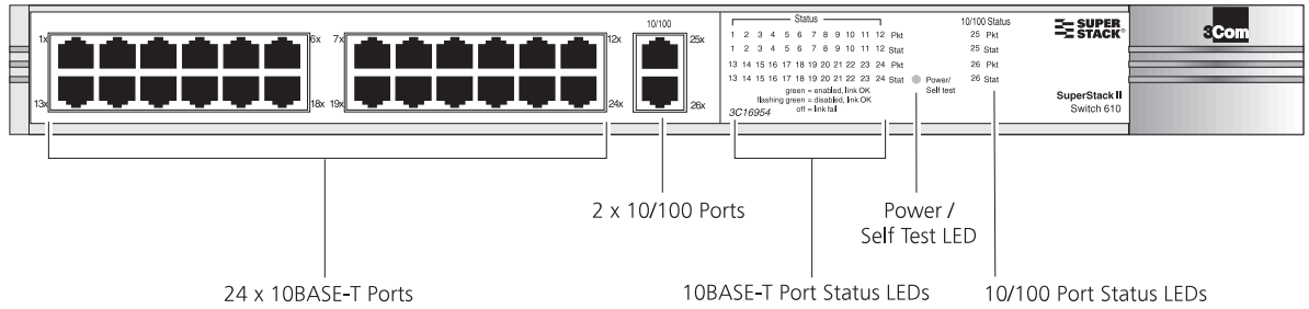
Figure 1 Switch 610 — Front view
