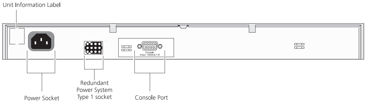
Figure 2 Switch 610 — Rear view
